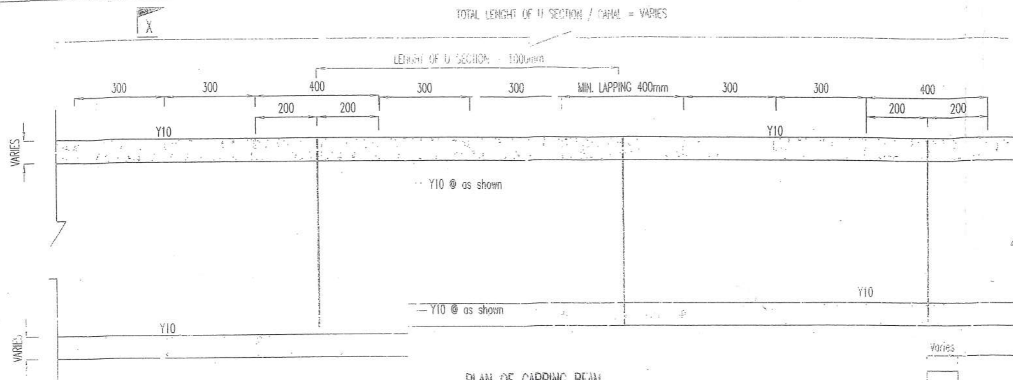
PLAN OF CAPPING BEAM
