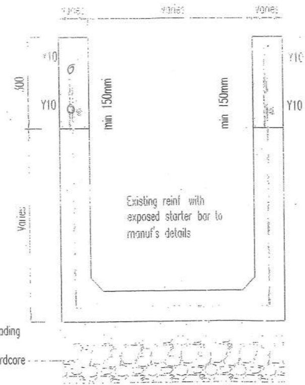
TYPICAL DETAIL OF U-SECTION WITH CAPPING BEAM-300mm HIGH
