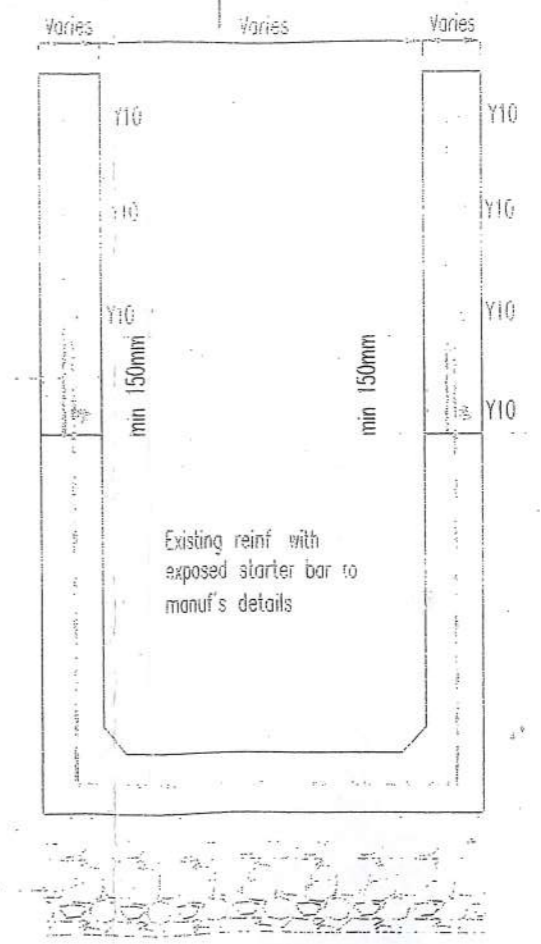
TYPICAL DETAIL OF U-SECTION WITH CAPPING BEAM-450mm HIGH
