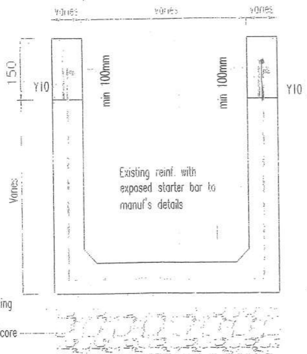
TYPICAL DETAIL OF U-SECTION WITH CAPPING BEAM-150mm HIGH
