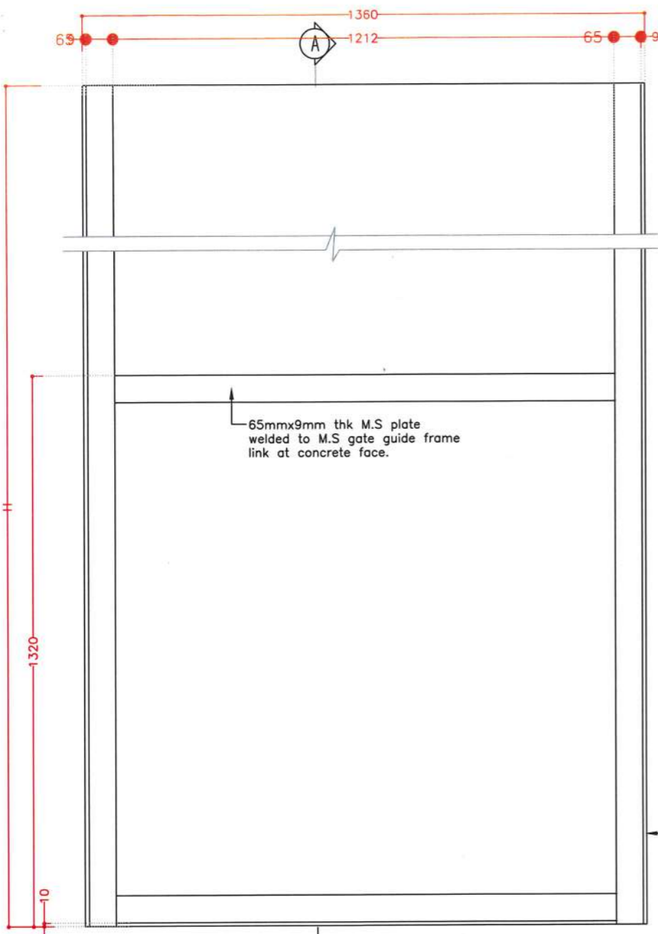
ELEVATION OF GATE FRAME
