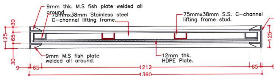
SECTIONAL PLAN
