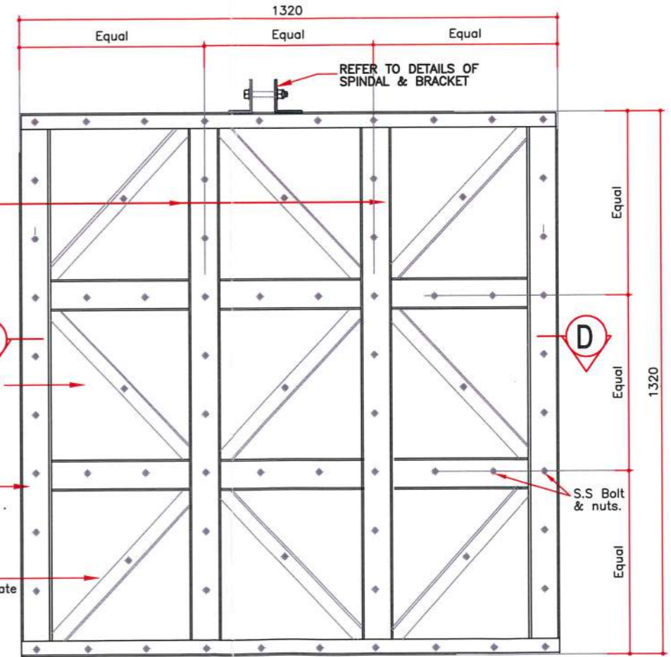
BACK ELEVATION HDPE LIFTING DEVICE FRAME (scale 1:25)
