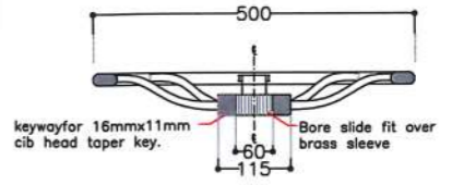
DETAILS OF G.I HANDWHEEL
