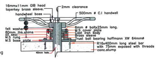
SECTIONAL ELEVATION
