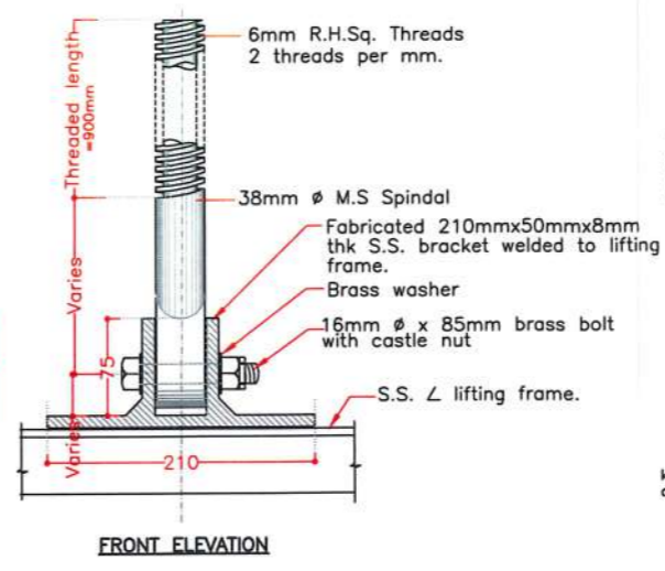
DETAIL OF M.S SPINDAL & BRACKET scale 1: 50
